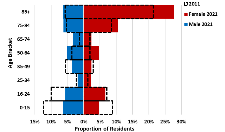
Proportion of Residents Living in Communal Establishments by Sex and Age Bracket in Stroud, 2011 and 2021
