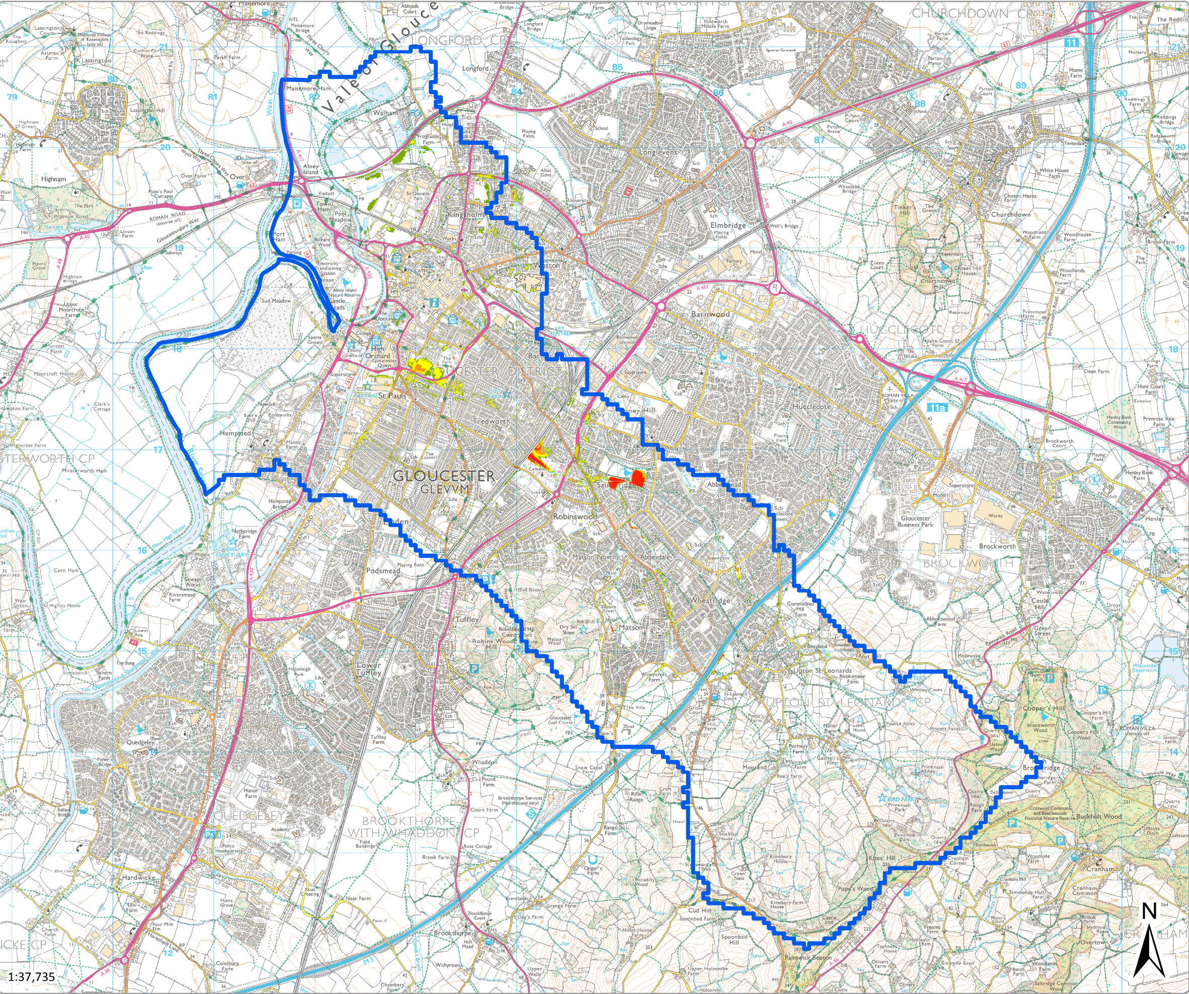
Central Gloucester SWMP 1 in 100 year event
