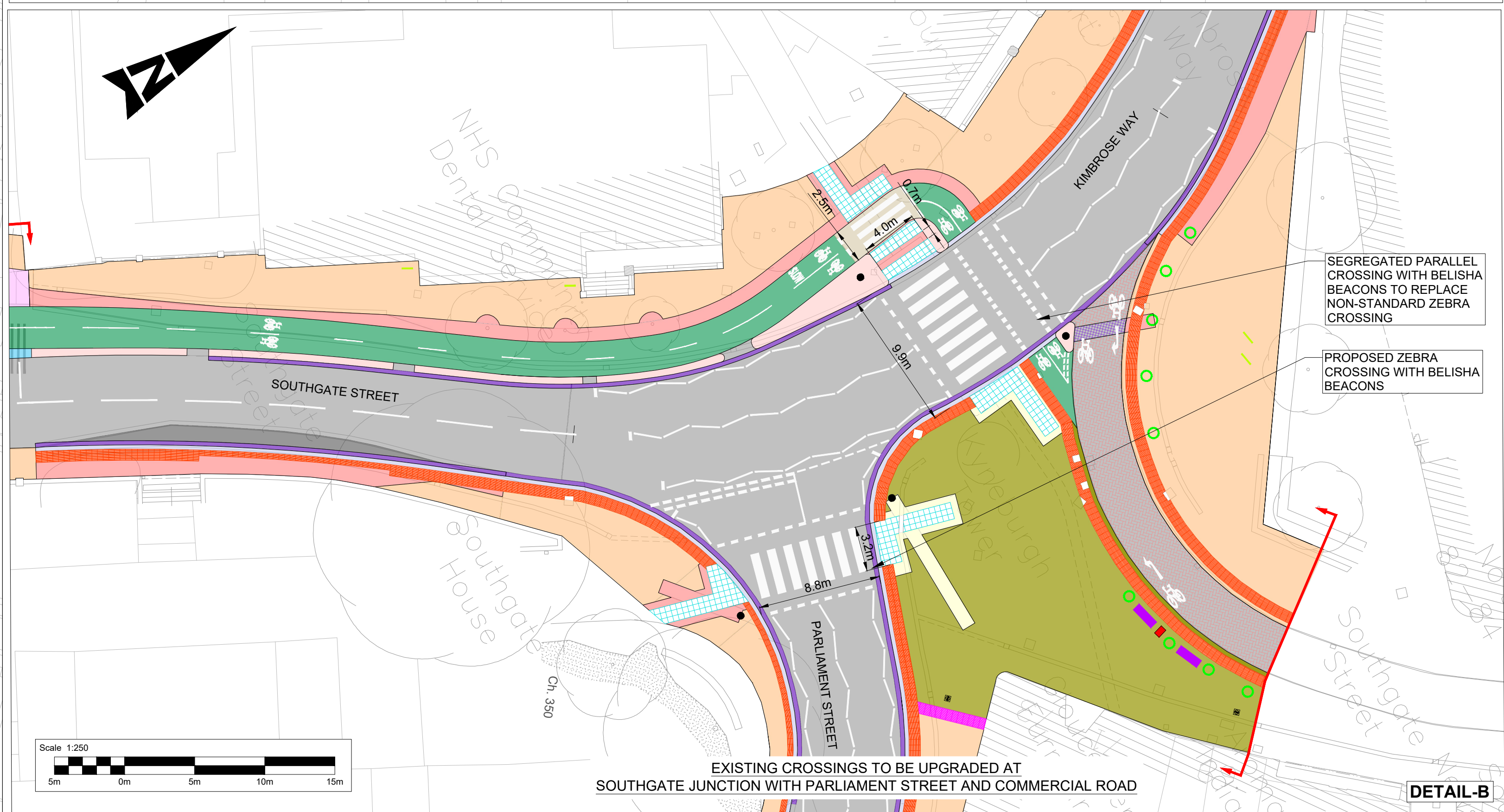
DETAIL-A
