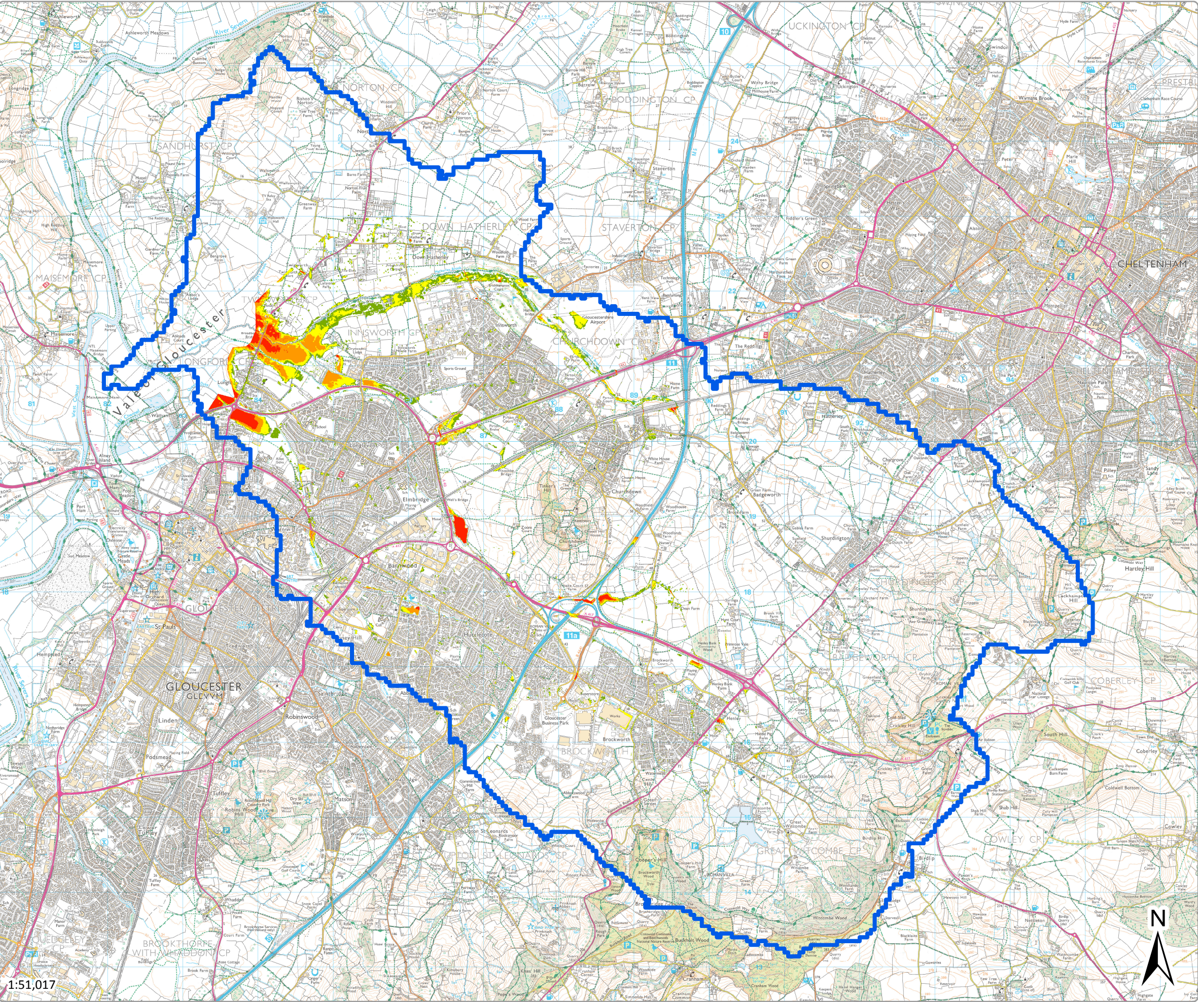
North Gloucester SWMP 1 in 200 year event
